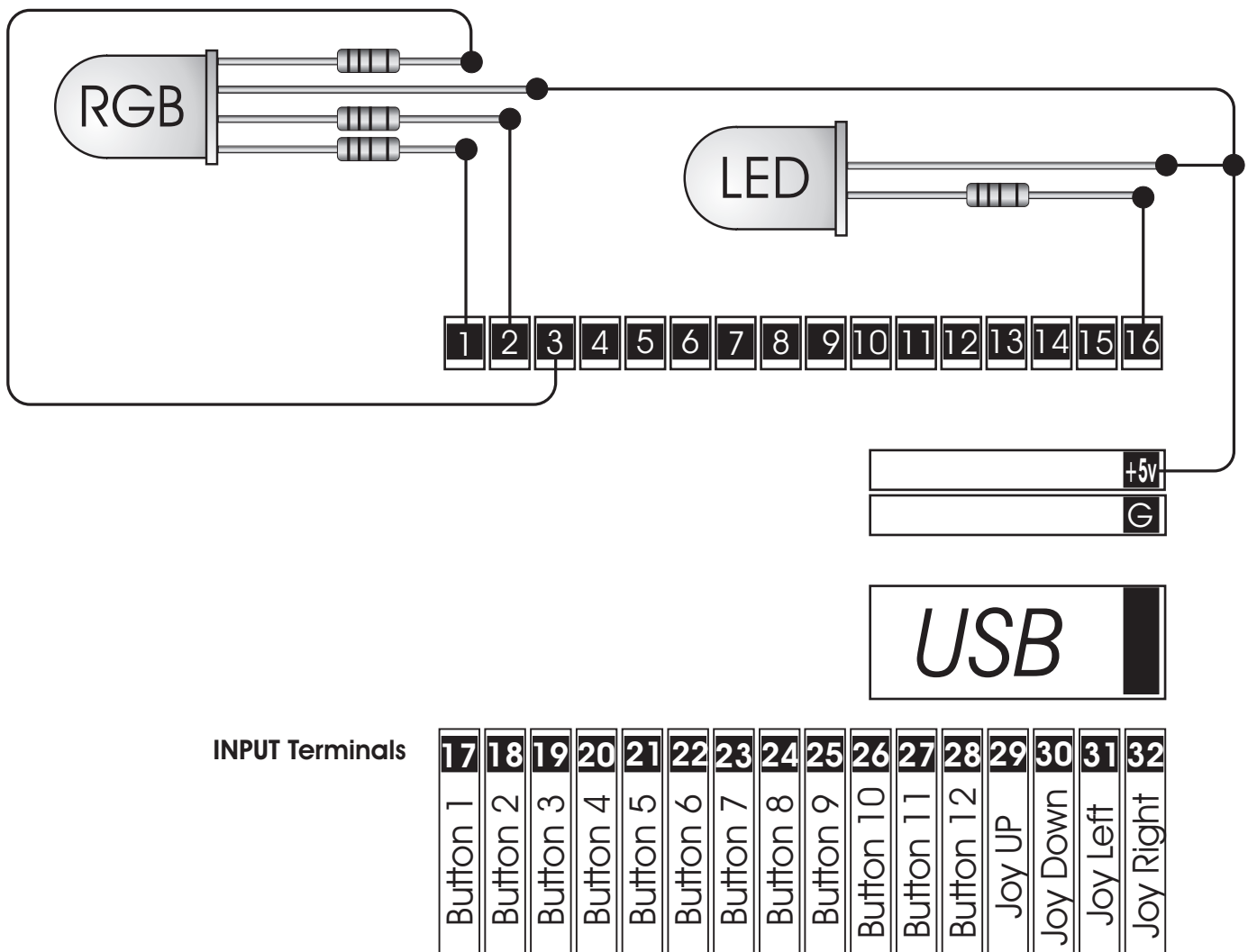
FIGURE 3. Example showing proper wiring of an RGB and Standard LED on OUTPUT side, and game controller assignments on INPUT side.
